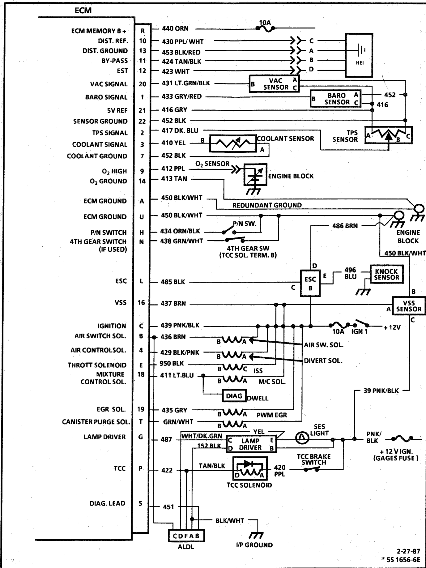
Figure A-6 - ECM Wiring Diagram - 5.0L (VIN H/G) & 5.7L (VIN 6)
