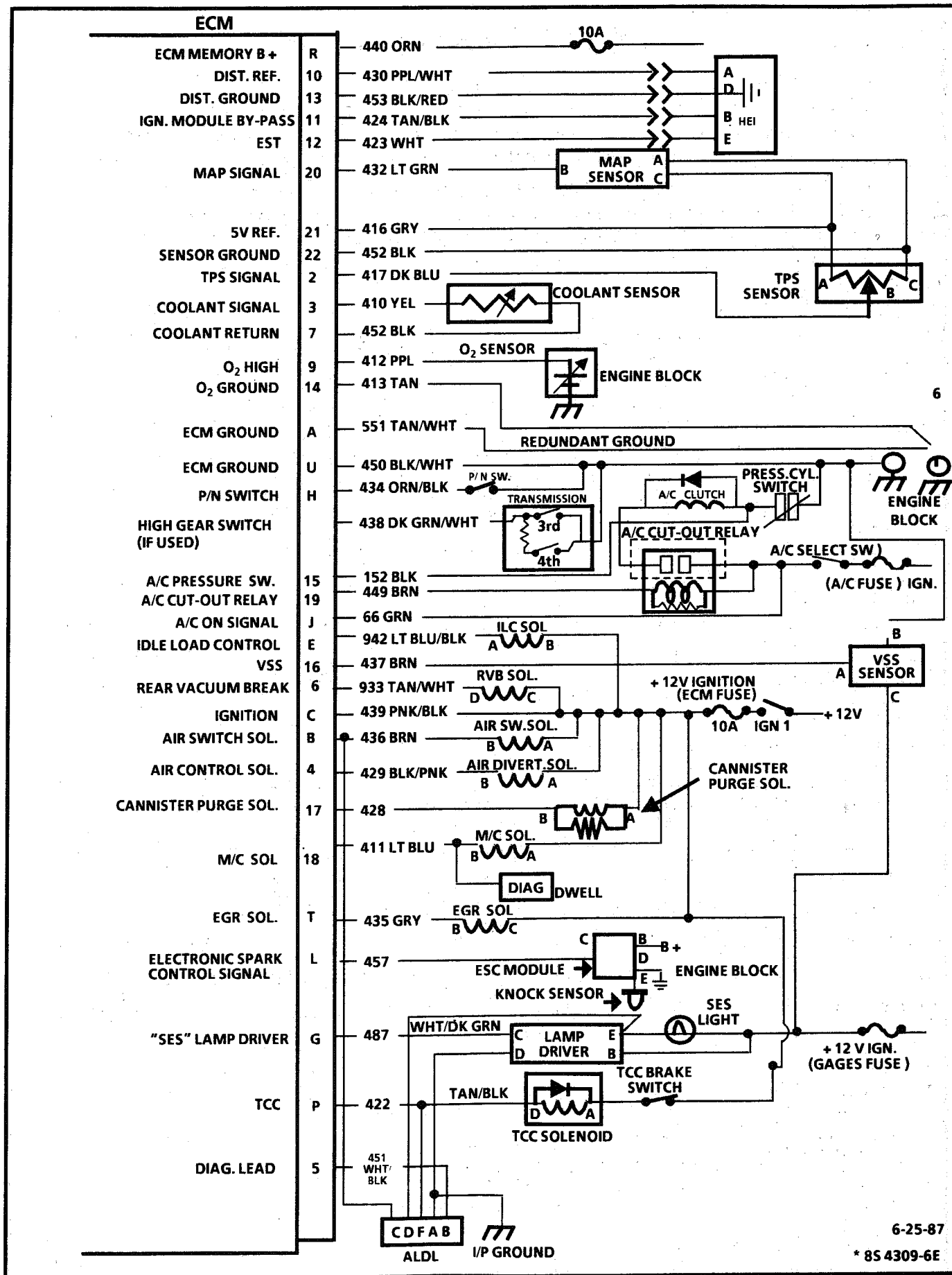
Figure A-4 - ECM Wiring Diagram 5.0L (VIN Y)
