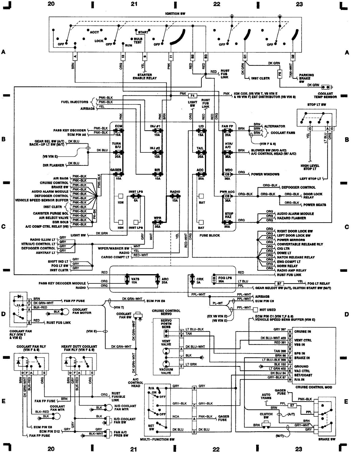
Fig. 6: Fuse Block (Grid 20-23) 1990 Chevrolet Camaro
