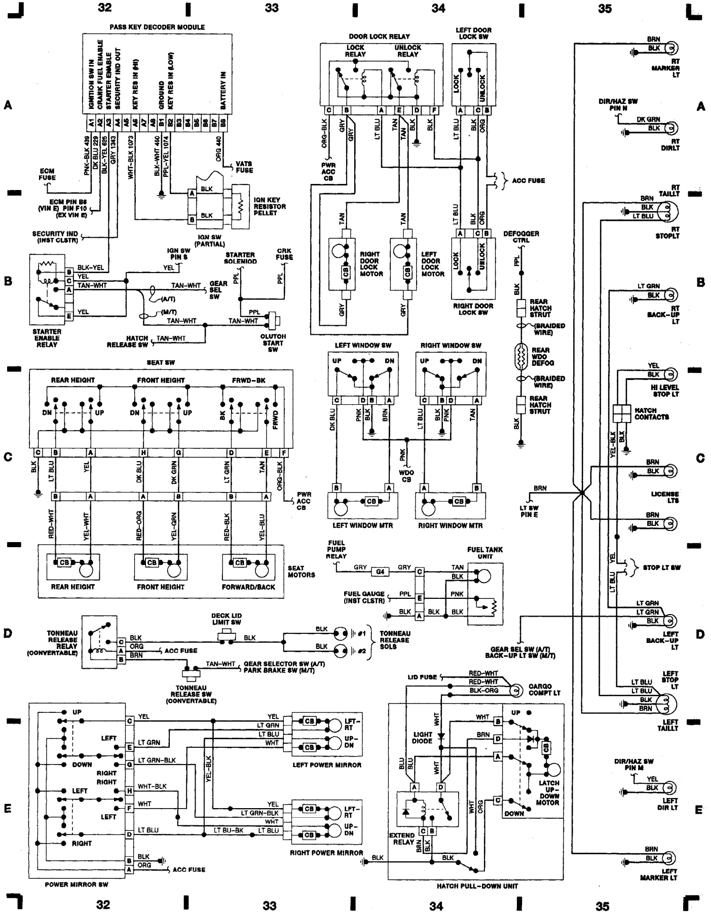
Fig. 9: Passenger Compartment & Taillights (Grid 32-35) 1990 Chevrolet Camaro
