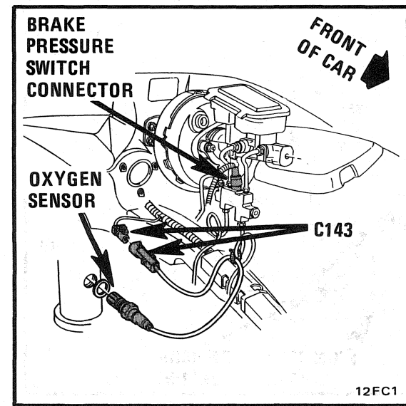
Figure C - LH Rear Of VIN F Engine Compartment (VIN 8 Similar)
