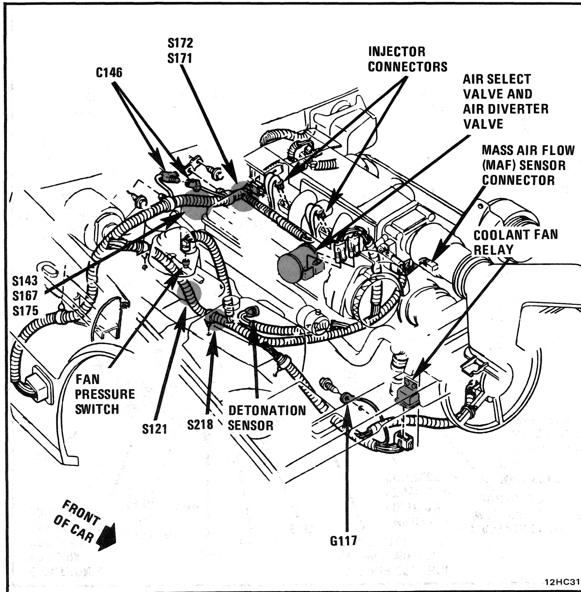
Figure A - RH Side Of VIN F Engine (VIN 8 Similar)
