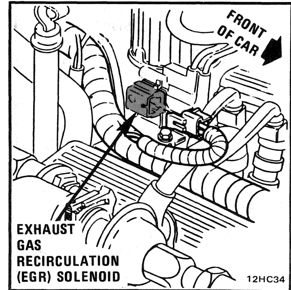
Figure B - Top RH Side Of VIN F Engine (VIN 8 Similar)
