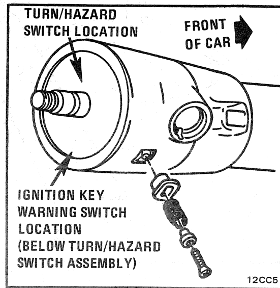
Figure C - Steering Column
