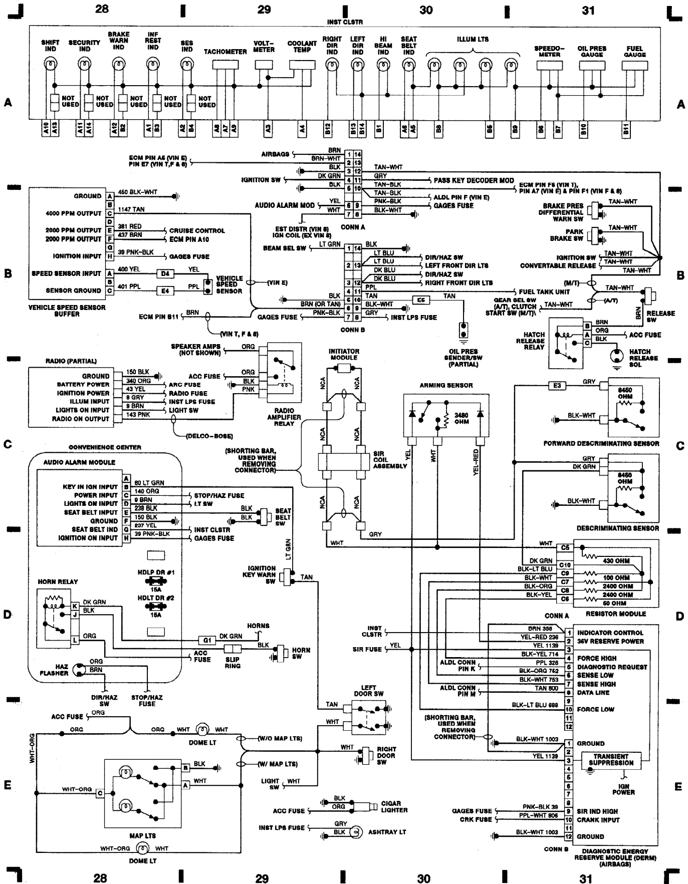
Fig. 8: Instrument Cluster, Vehicle Speed Sensor & Airbags (Grid 28-31)
