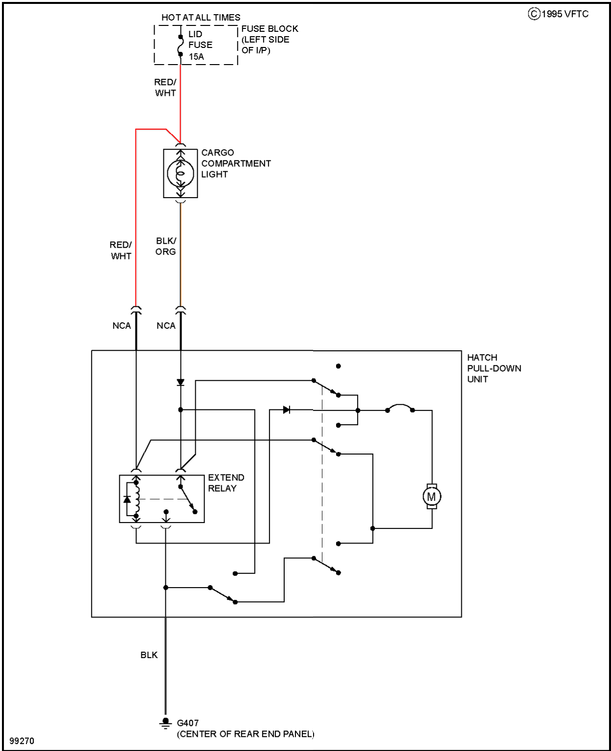
Fig. 17: Hatch Pull-Down Circuit
