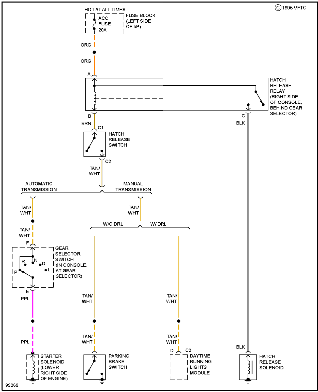
Fig. 18: Hatch Release Circuit
