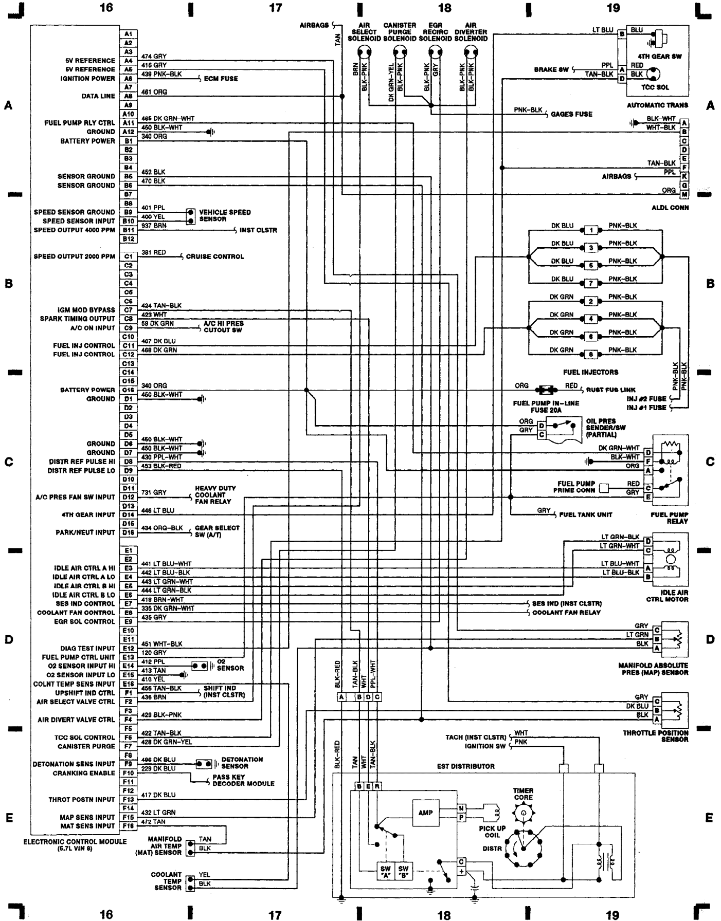
Fig. 5: Electronic Control Module (5.7L VIN 8) (Grid 16-19) 1990 Chevrolet Camaro
