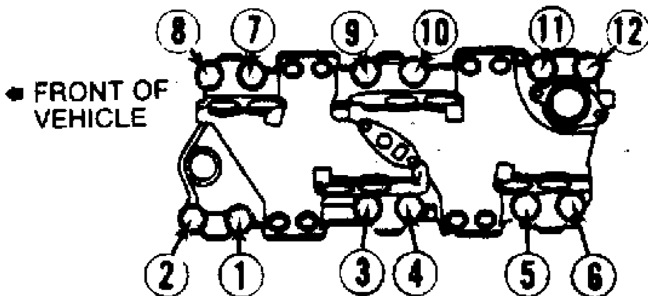
Final Tightening Sequence
