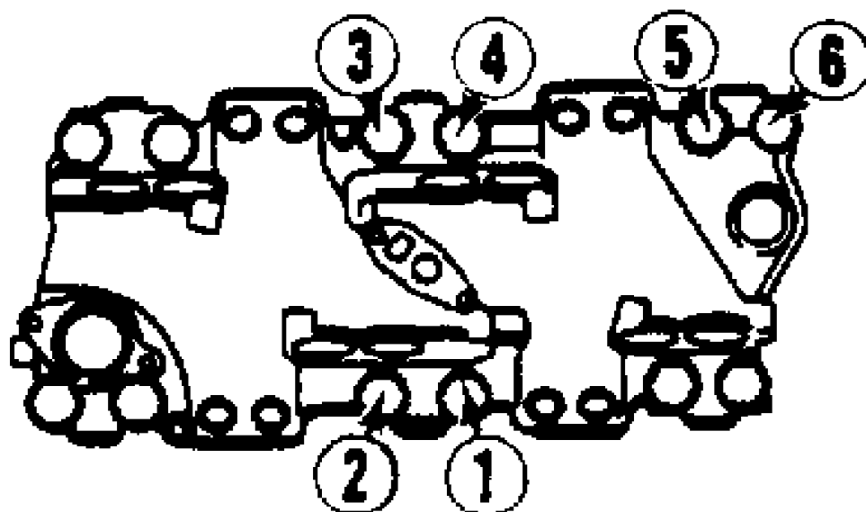
Snug Tightening Sequence
