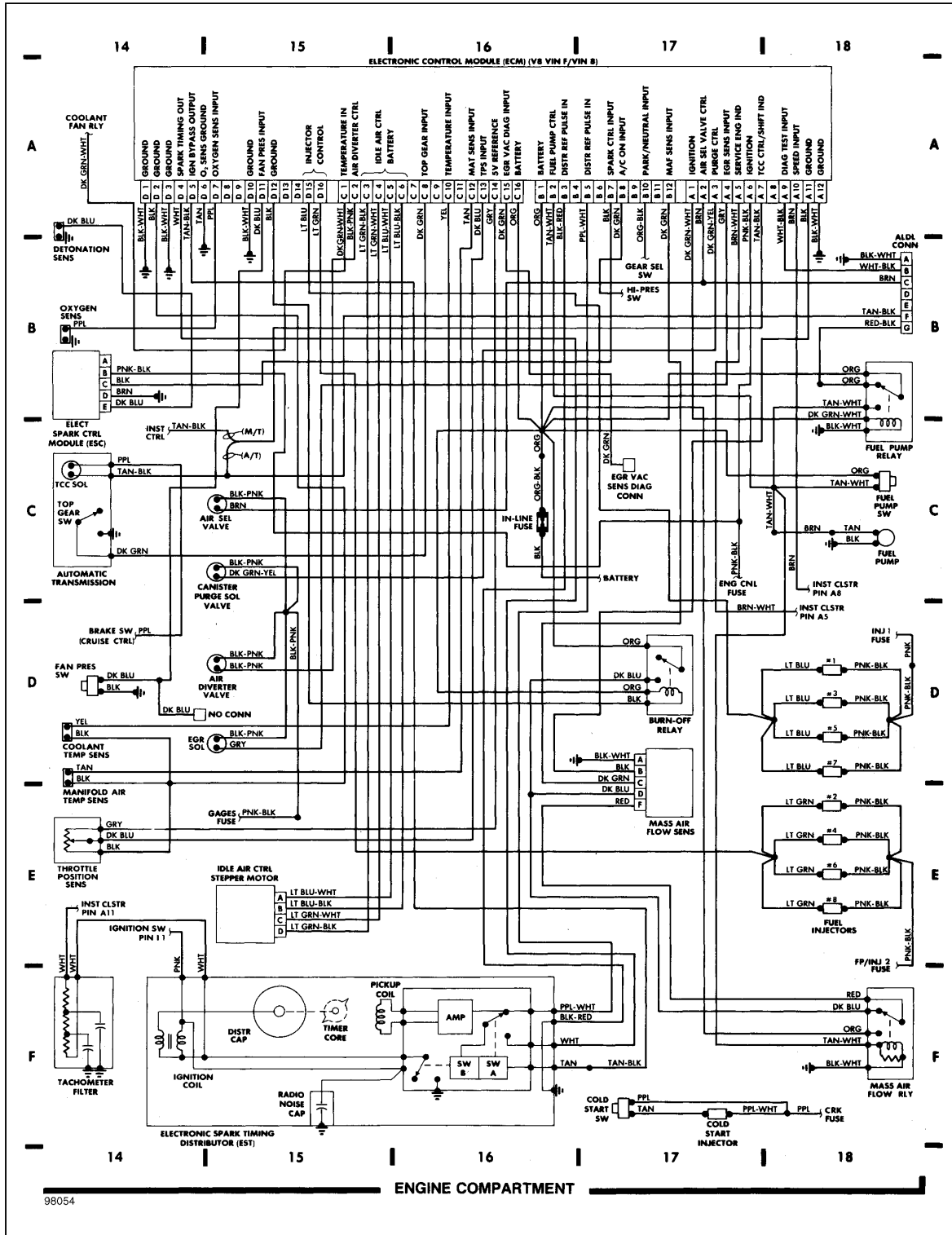
Fig 4: Engine Compartment (Cont.)
